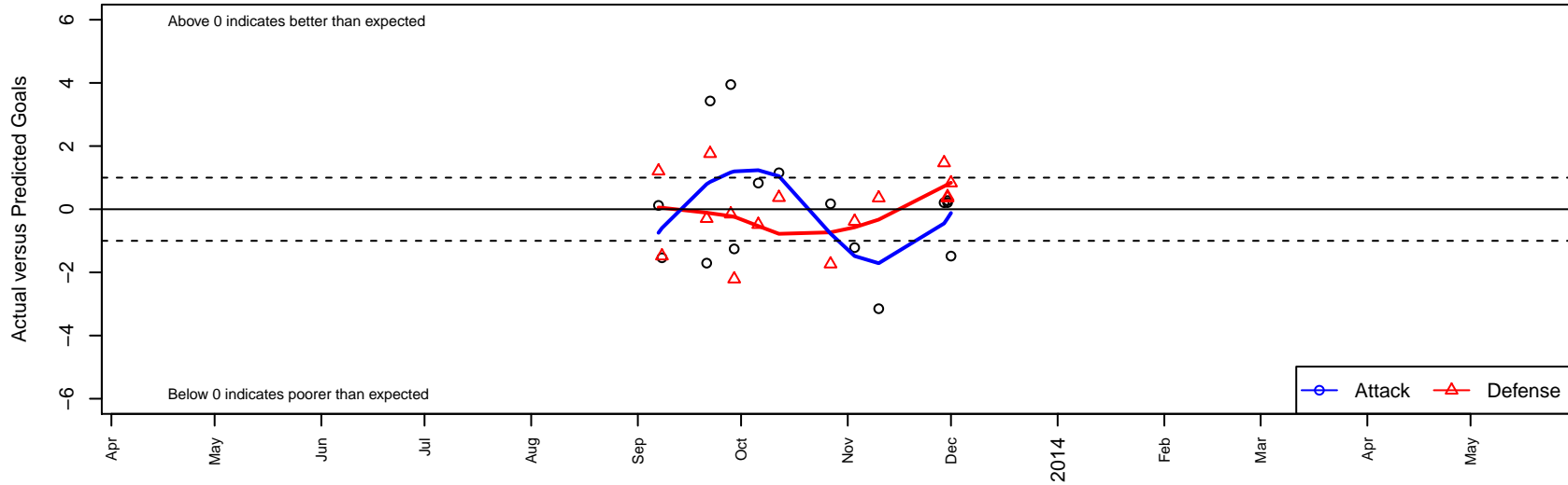
Eagles SC B94 Dots are actual minus expected GF (blue circles) and GA (red triangles). Blue line is smoothed change in attack strength. Red is smoothed change in defense strength.
